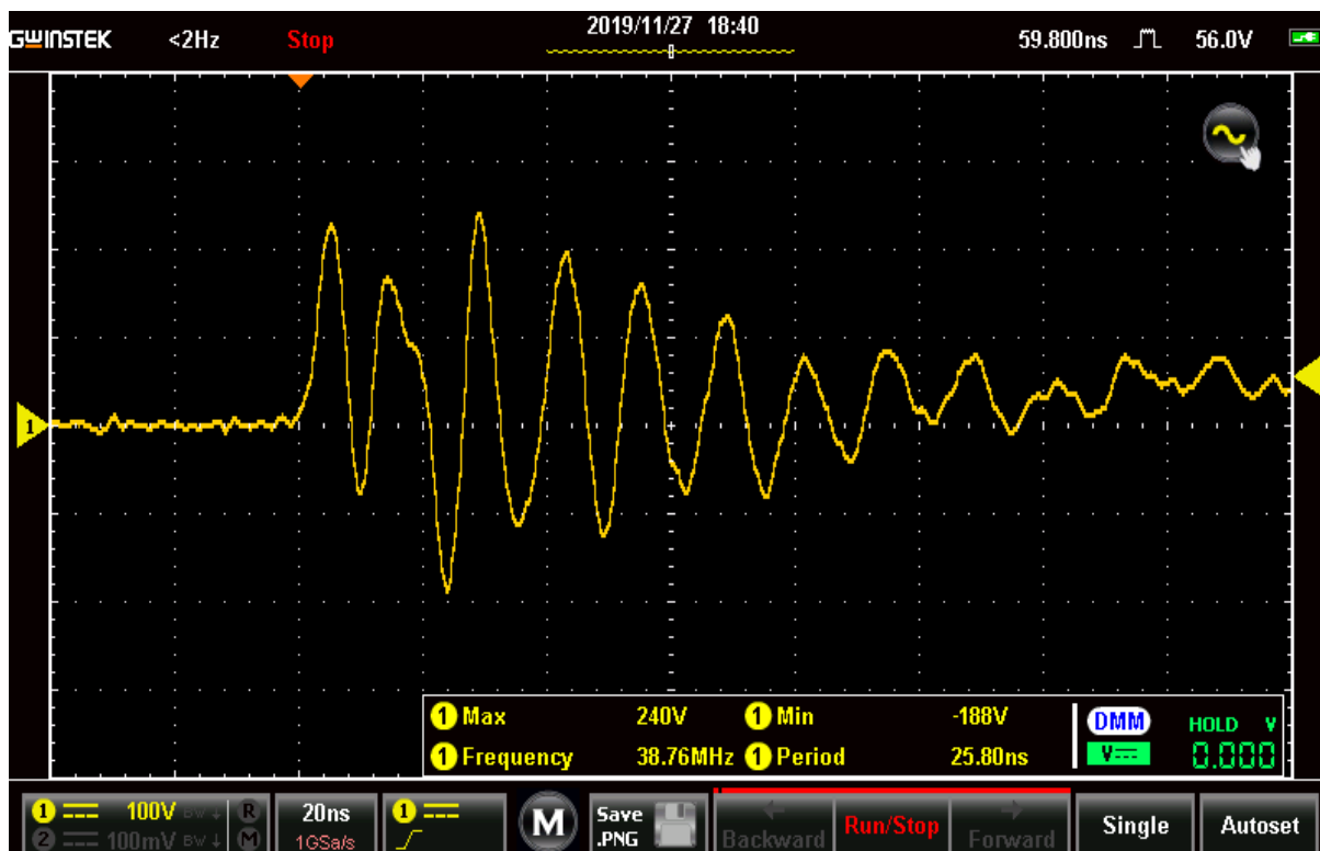
Fig. 2 Oscilogram residual overvoltage u(t) on the protected output of the band coaxial overvoltage protection PKOpt-N-lambda-0,9G-BCD/F-F in the shock current test 2,5 kA,
